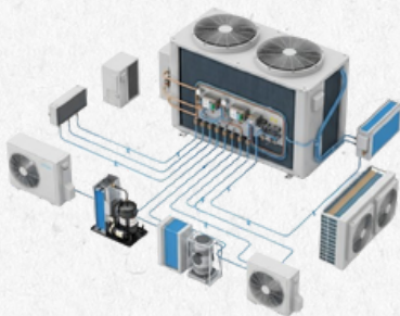
VRF System
